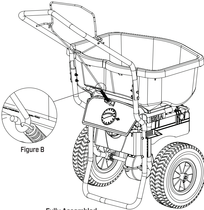
Fully Assembled
