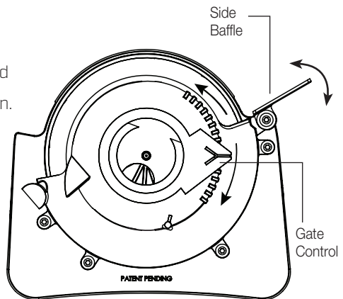
FIGURE C (Gate Location)
